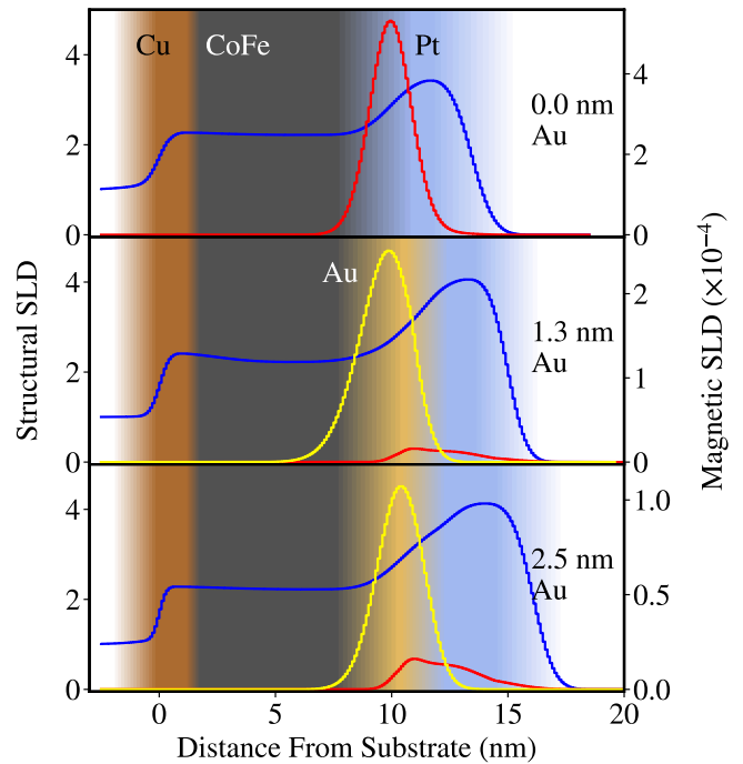
FIG. 10. Structural (blue) and magnetic (red and yellow) scattering length densities from the model fits to the magnetic reflectivity data for varying Au spacer layer thicknesses, indicated on the figure. The red line indicates the extent of the induced Pt moment and the yellow the extent of the induced Au moment. Note the mSLD axes have different scales.
