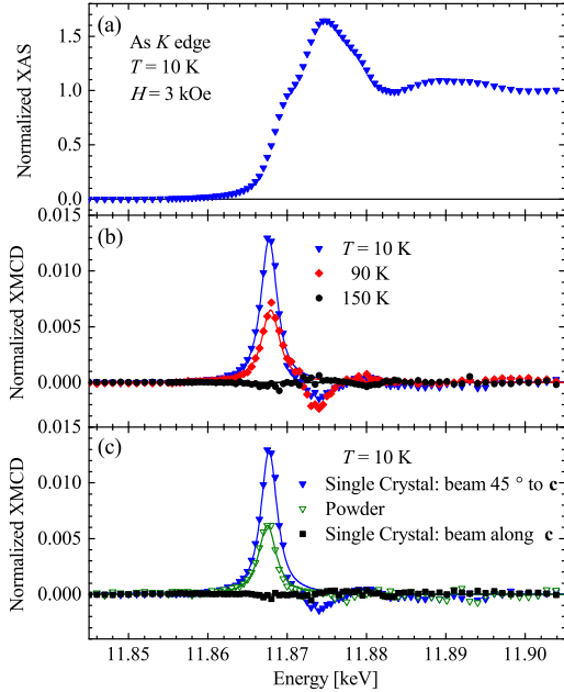
FIG. 1 (color online). (a) The normalized XAS signal across the As K edge from transmission measurements made on a single-crystal sample. The XAS signal has been normalized to 1 at energies well above the edge. (b) Edge-step normalized XMCD data for H = 3 kOe and various temperatures taken with the crystal's c axis oriented 45^\circ away from the incoming beam ( H_{ab} = 2.1 kOe). The T = 10 K data relate to the XAS data in (a). (c) Edge-step normalized XMCD data for T = 10 K and H = 3 kOe taken across the As K edge for powder and single-crystal samples. Data for the single crystal are shown for the c axis oriented either at 45^\circ to the incoming beam or parallel to the beam. The colored lines in (b) and (c) are fits to Lorentzian line shapes.
