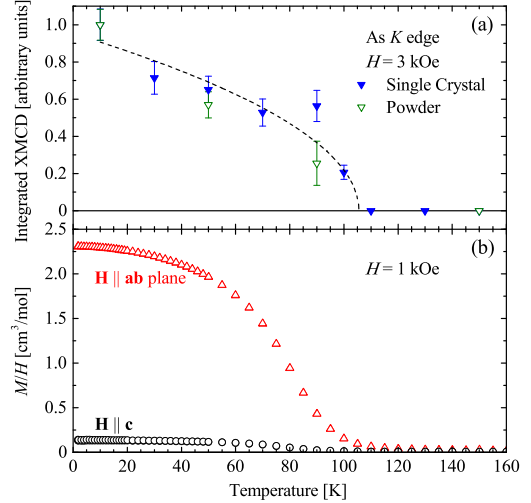
FIG. 2 (color online). (a) The temperature dependence of the integrated XMCD signal for the H = 3 kOe As K edge XMCD data. Data are shown for both a single-crystal sample with its c axis oriented 45^\circ away from the incoming beam and a powder sample. The integrated XMCD signal has been determined from fits to the peak in the XMCD data with a Lorentzian line shape. Both data sets are normalized to their values for T = 10 K, and the dashed line is a guide to the eye. (b) \chi = M/H data for \text{Ba}_{0.6}\text{K}_{0.4}\text{Mn}_2\text{As}_2 from Ref. [12]. The nonzero value of \chi as T \rightarrow 0 for \mathbf{H} applied parallel to the c axis is due to a slight misalignment of the crystal ( \approx 4^\circ ) [12].
