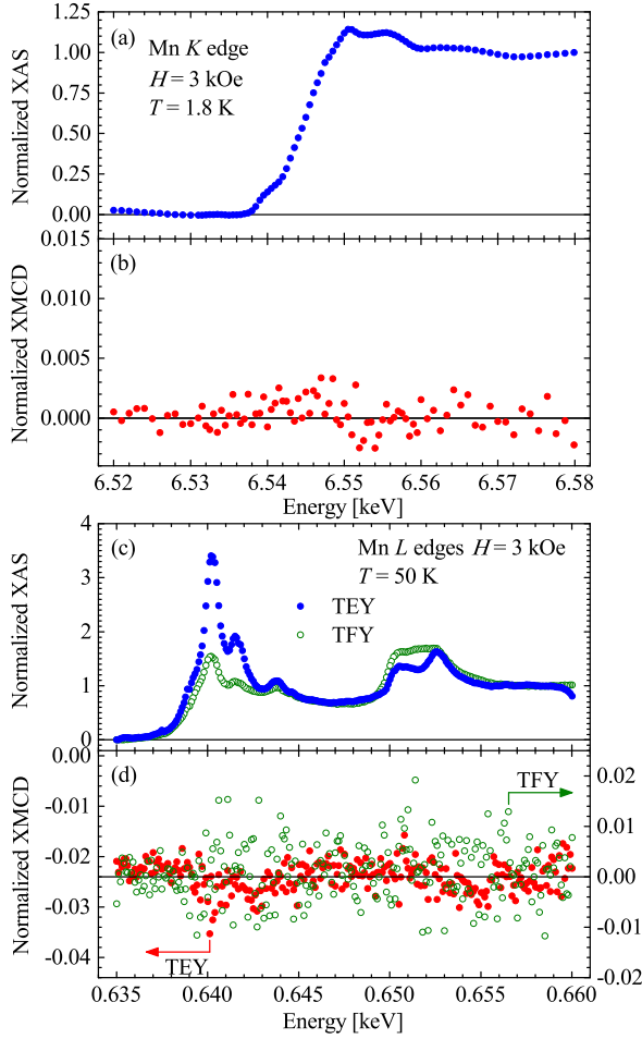
FIG. 3 (color online). (a) The normalized XAS signal across the Mn K edge for T = 1.8 K and H = 3 kOe from transmission measurements made on a single-crystal sample with its c axis oriented 45^\circ away from the incoming beam. (b) Normalized XMCD data corresponding to the XAS data in (a). (c) Normalized XAS data for T = 50 K and H = 3 kOe taken across the Mn L_2 and L_3 edges from measurements of the total electron yield and total fluorescence yield made on a single-crystal sample with its c axis oriented 70^\circ away from the incoming beam ( H_{ab} = 2.8 kOe). (d) Normalized XMCD data corresponding to the TEY (left axis) and TFY (right axis) data in (c). The small constant offset in the TEY data is due to leakage currents and currents induced by external electromagnetic fields in the leads connected to the picoammeter used for the measurements. The TFY data in (c) and (d) have not been corrected for absorption of the fluoresced x rays by the sample [31].
