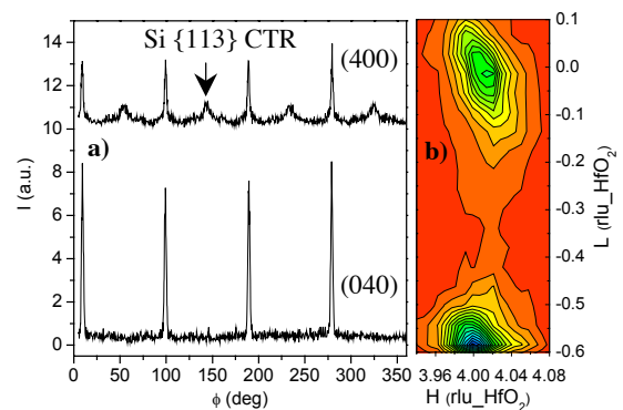
Fig. 2. a) \phi scans across m-HfO 2 {400} and {040} reflections. b) a K-L mesh scan near m-HfO 2 (400) surface reflection.
