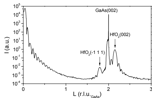
Fig. 1. \theta - 2\theta scan along surface normal.
