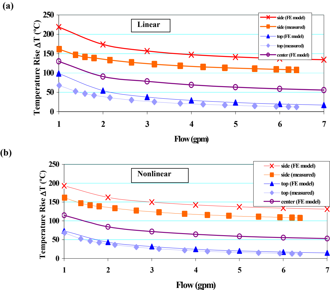
Fig. 4: Comparison of experimental and FE results for different flow values. Effect of wall temperature on h_f ignored in (a) and included in (b).
