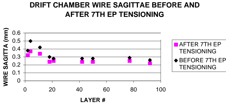
Figure 8: KLOE drift chamber wire sagittae calculated from the measurement of wire mechanical tension, obtained independently of survey.
