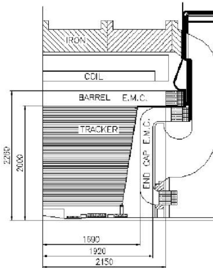
Figure 2: one quarter cross sectional view of KLOE, showing approximate dimension and location of the four subsystems.
