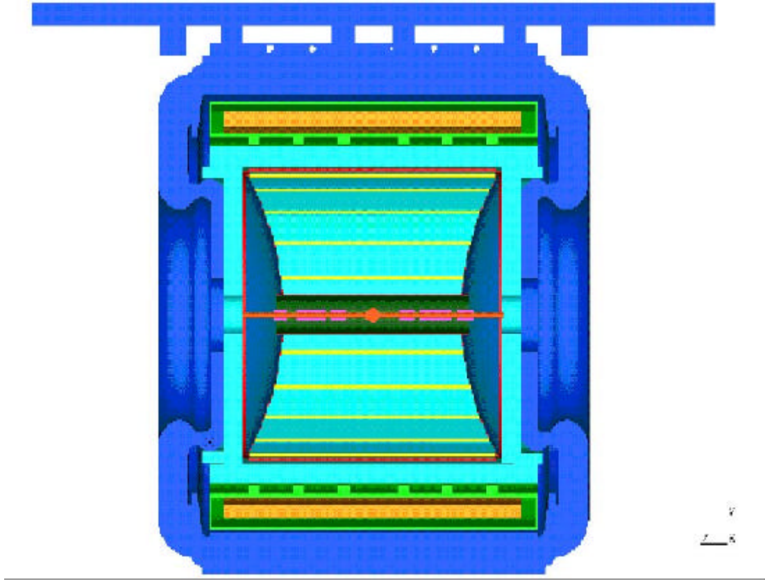
Figure 1: cross section of KLOE, showing (from inside to outside): spherical Be beam pipe, quadrupoles, carbon fiber drift chamber with spherical end plates, barrel plus end cap electromagnetic calorimeters, cryostat with superconducting coil and the iron return yoke, which encloses everything. On top are 4 flat iron platforms with engines for opening and closing the 4 yoke end cap halves.
