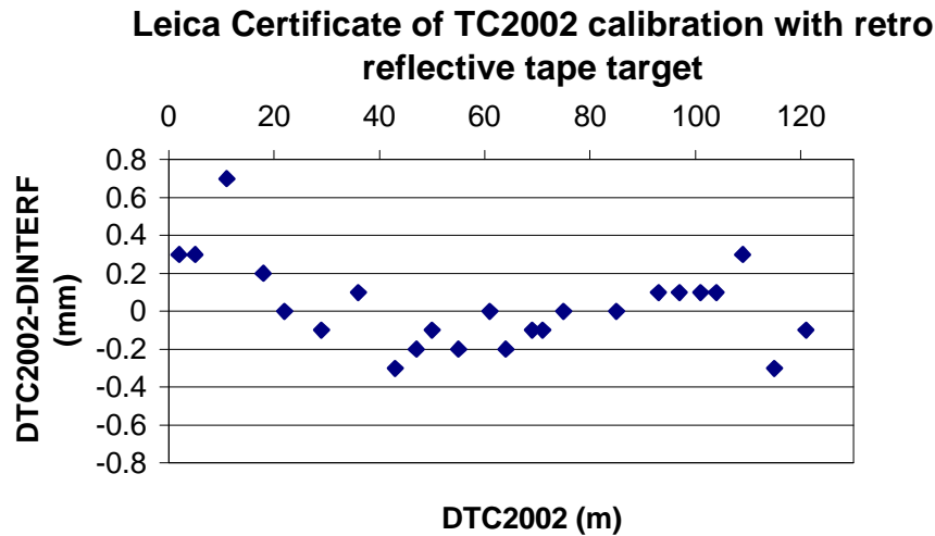
Figure 5: calibration of KLOE’s TC2002 with retro-reflective targets bought from Leica.
