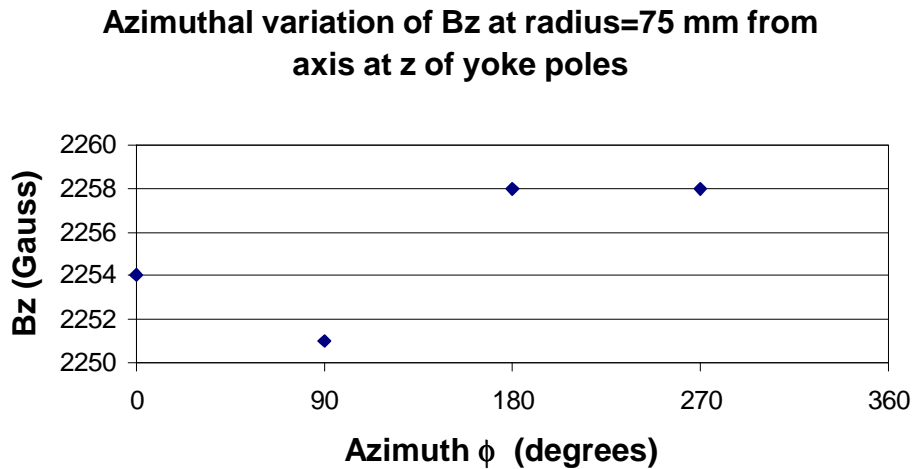
Figure 18: the small measured \phi -asymmetry of the field longitudinal component B_z in the yoke poles (2 Gauss in the vertical 0^\circ - 180^\circ plane and 3 Gauss in the horizontal 90^\circ - 270^\circ plane with respect to averages).
