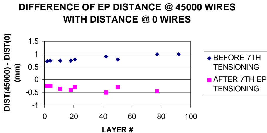
Figure 9: adjustment of the distance of the KLOE drift chamber end plates by end plate tensioning in order to control wire sagittae. Results are obtained independently from survey and are in agreement with TC2002 survey results.
