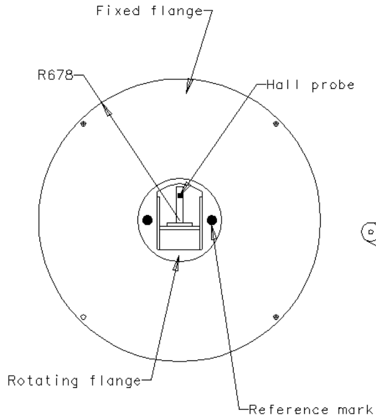
Figure 13: front view of DAΦNE's MagAx.
