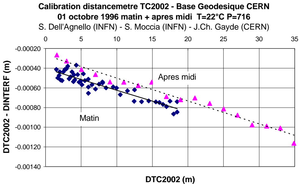
Figure 4: comparison of different calibrations of KLOE's TC2002 with 3D targets.
