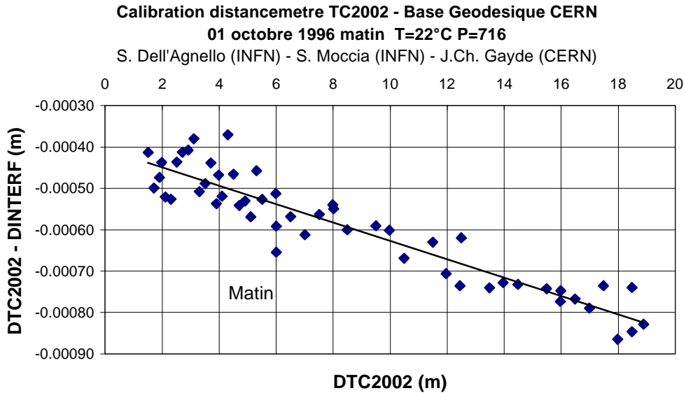
Figure 3: calibration of KLOE's TC2002 with 3D reflectors with CERN's interferometer.
