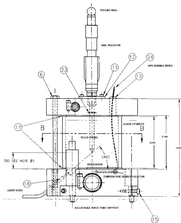
Fig. 2. Cross section of an HLS vessel.
