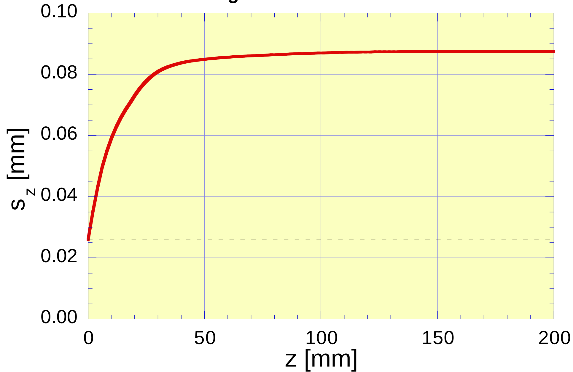
Bunch Length from Cathode to Gun Exit
