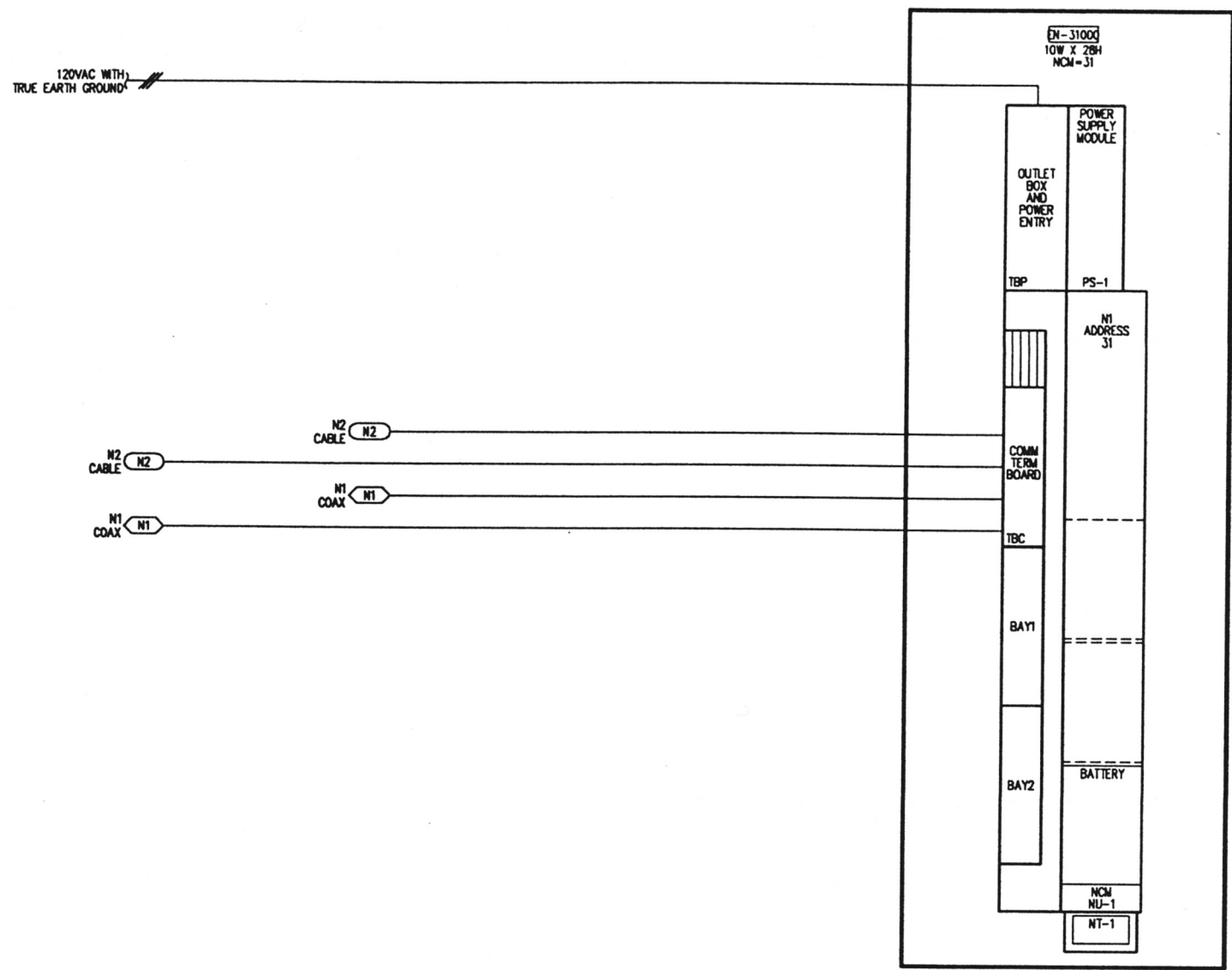
Enclosure, EN-31000, NCU Serving the Process Water Systems in Building 420
